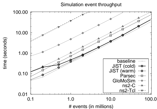
Figure 16: JiST has higher event throughput and comes within 20% of the baseline lower bound. The kink in the JiST curve (at left) in the first fraction of a second of simulation is evidence of JIT compilation at work. The table (at right) shows the time to perform 5 million events and also normalized against both the baseline and JiST performance.
