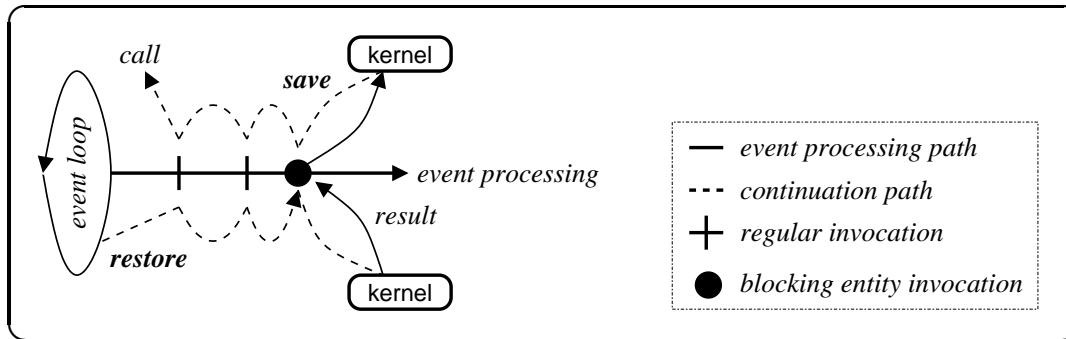
Figure 13: The JiST event loop also functions as a continuation trampoline. It saves the continuation state on a blocking entity method invocation and restores it upon receiving the callback. Due to Java constraints, the stack must be manually unwound and preserved.
